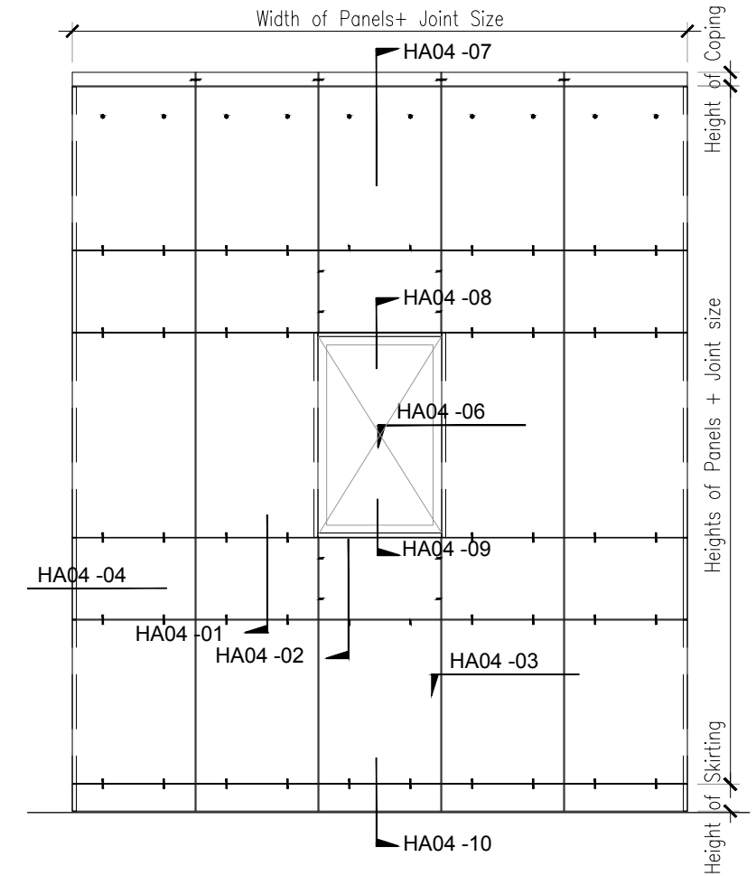
Elevation Scale 1:50
