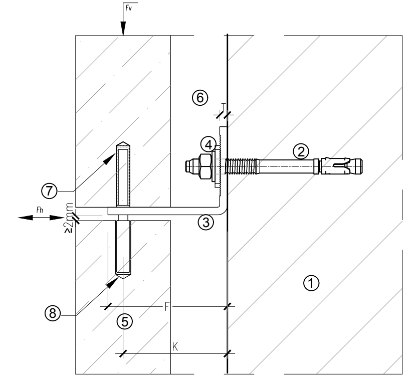
Vertical section Scale 1:2
