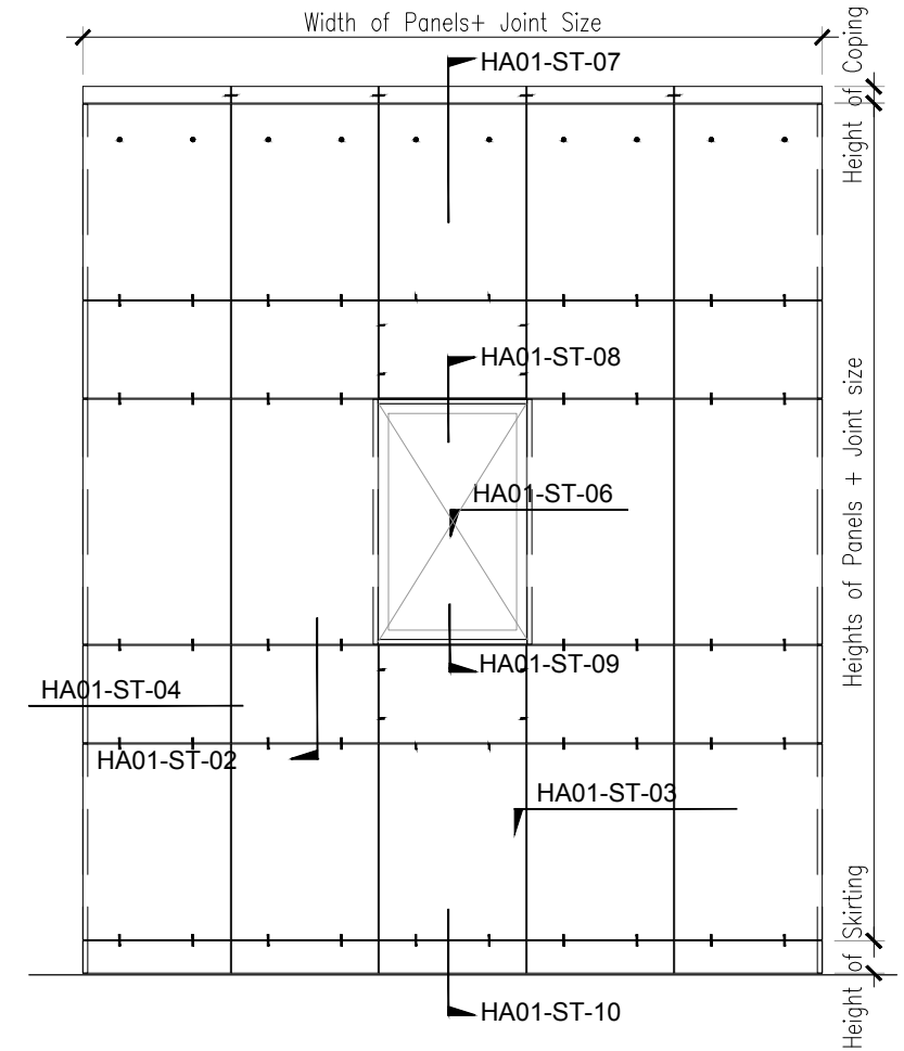
Elevation Scale 1:50
