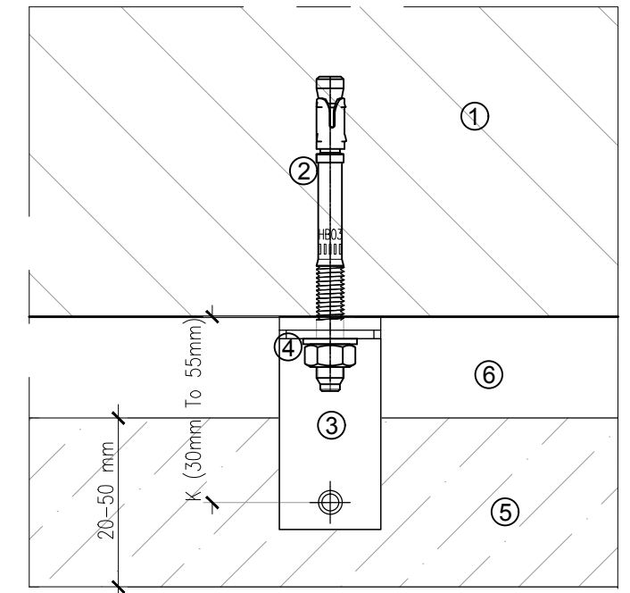
Horizontal Section Scale 1:2
