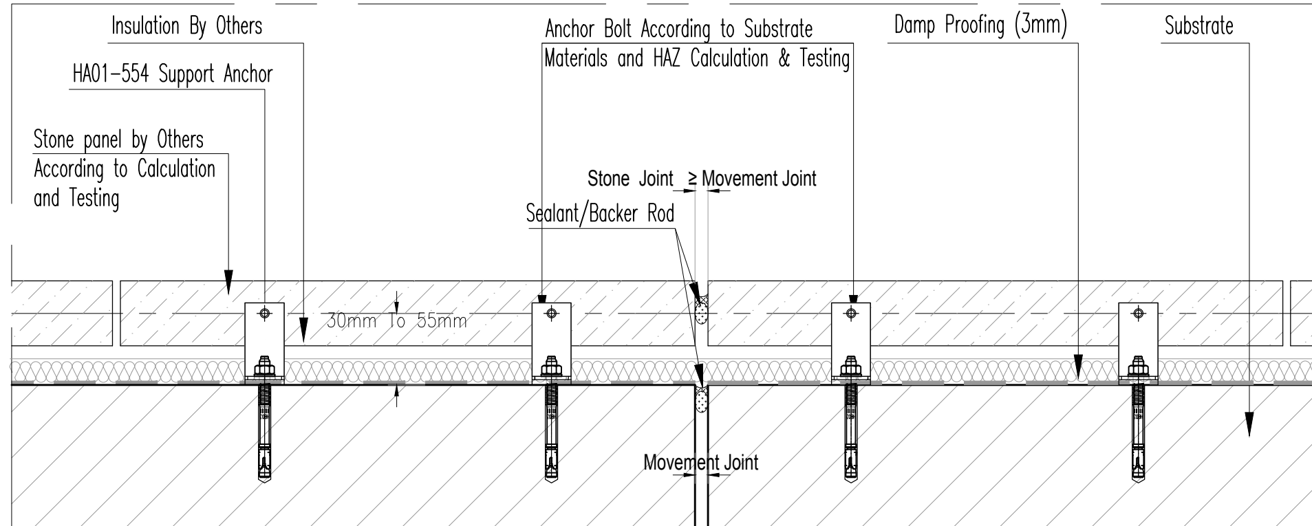
Horizontal section Scale 1:4
