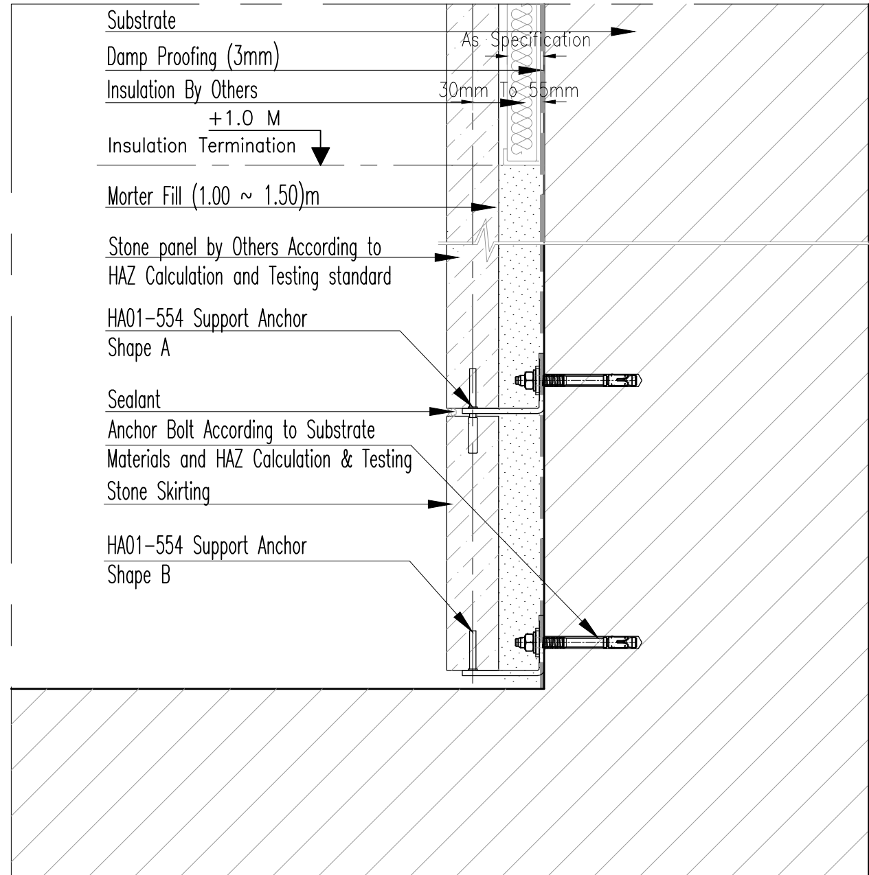
Vertical section Scale 1:4
