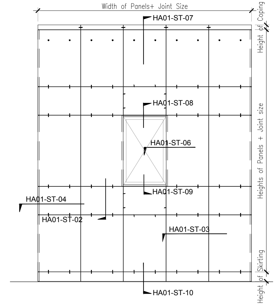
Elevation Scale 1:50
