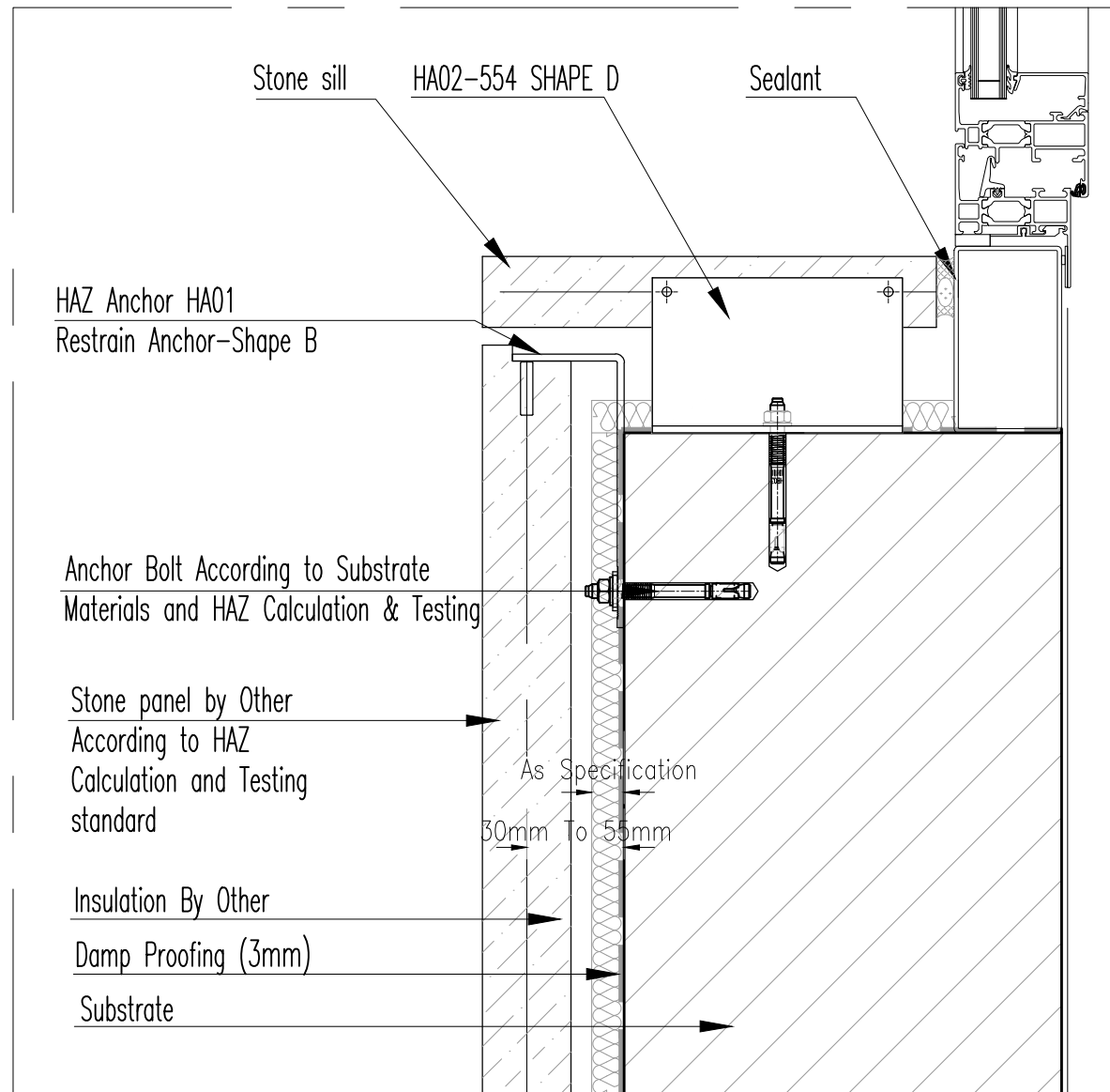
Vertical section Scale 1:4
