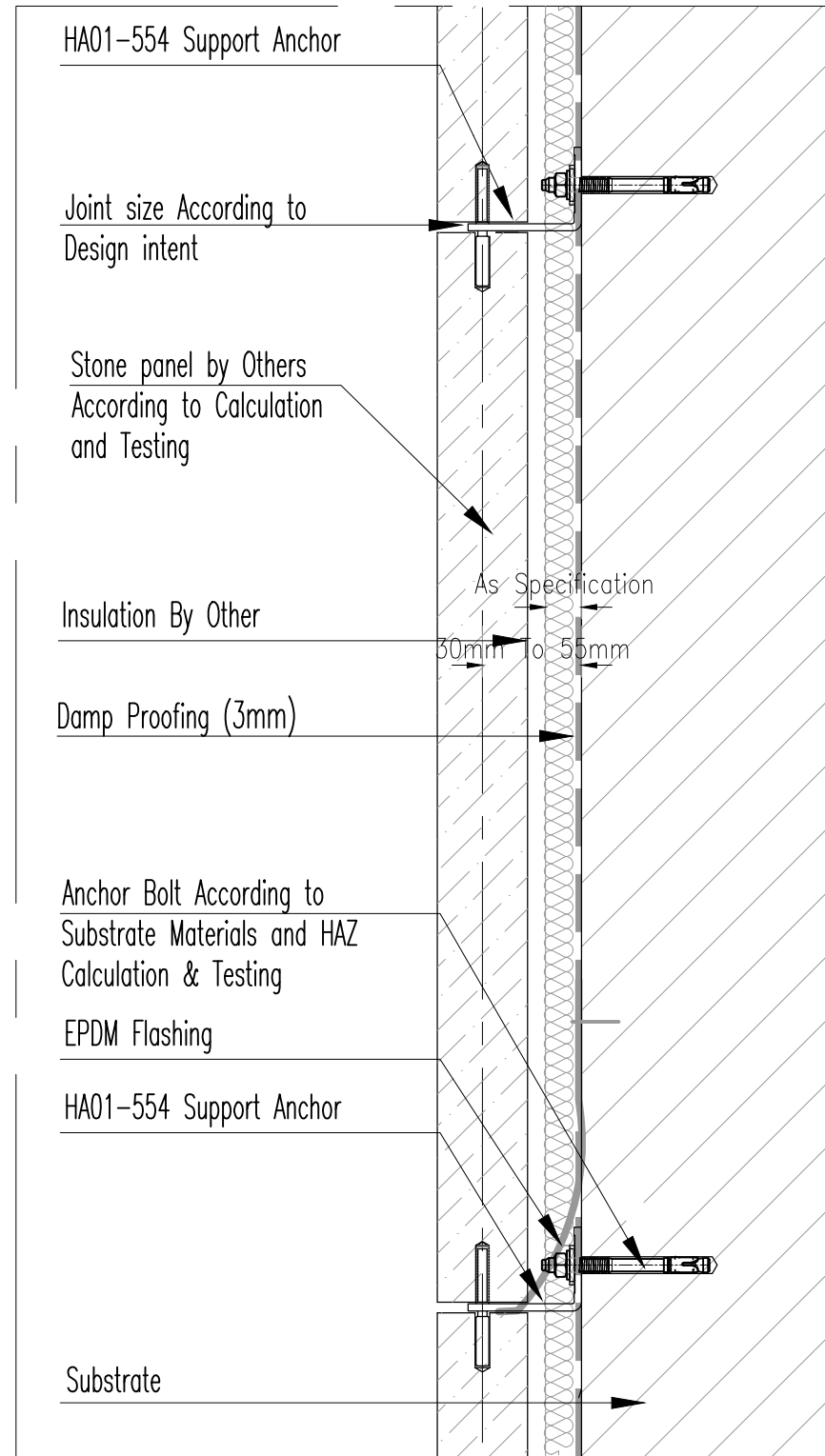
Vertical section Scale 1:4
